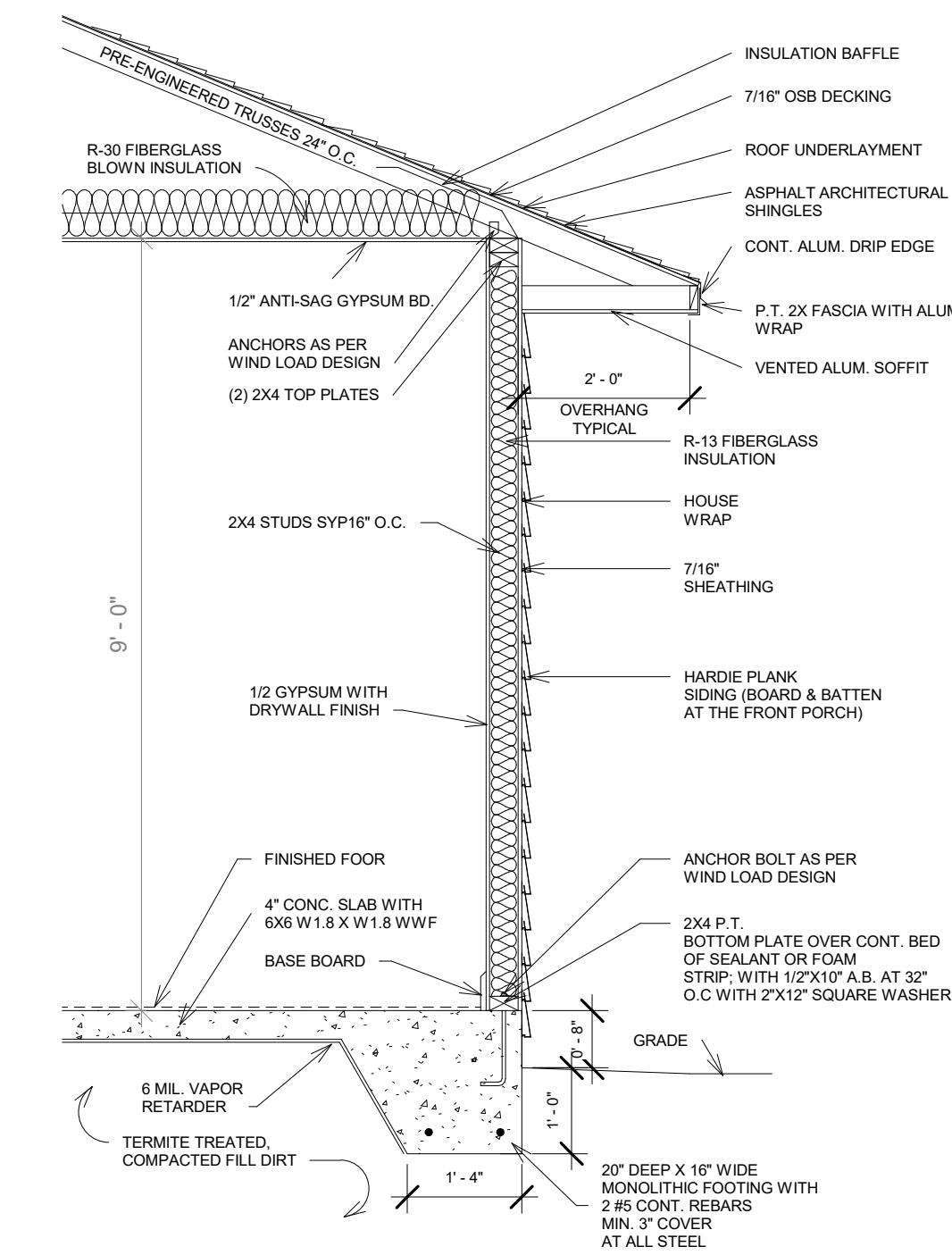
2 TYPICAL WALL SECTION 1/2" = 1'-0"
